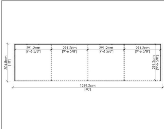
1 TOP VIEW
