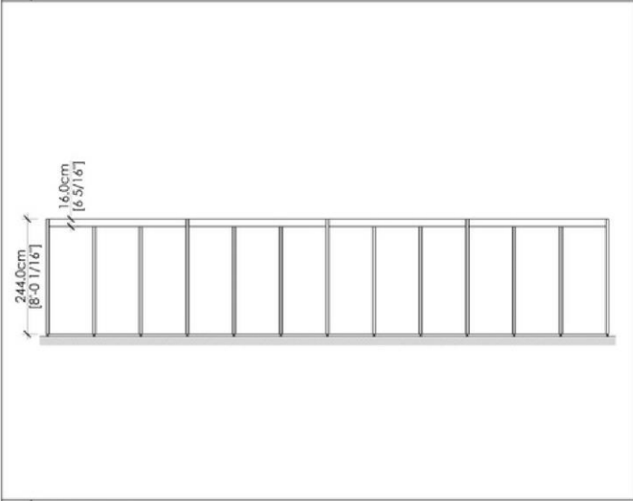
2 FRONT VIEW
