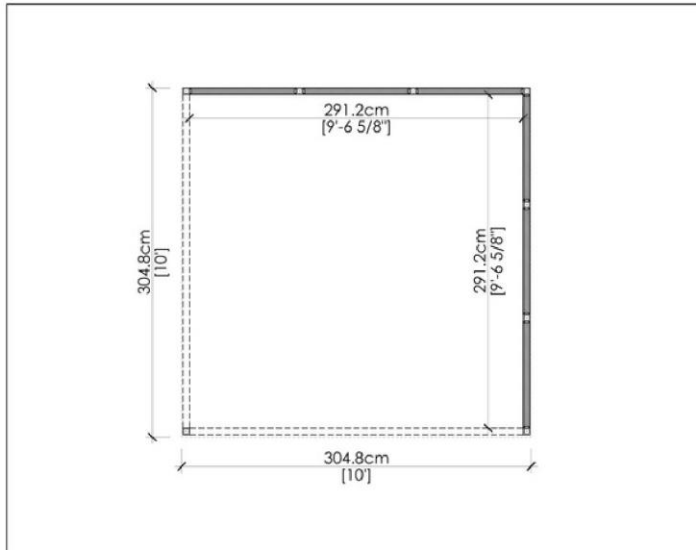
1 TOP VIEW
