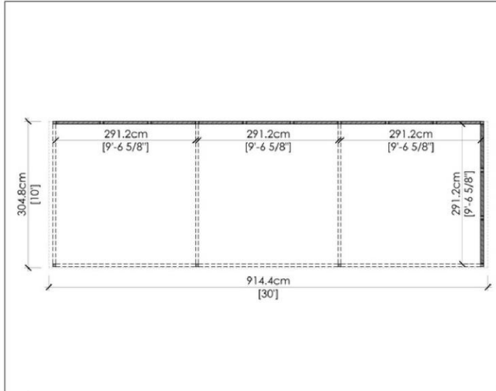
1 TOP VIEW
