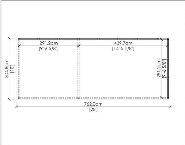
1 TOP VIEW
