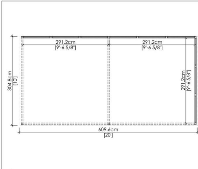
1 TOP VIEW
