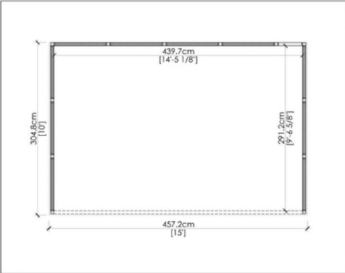
1 TOP VIEW
