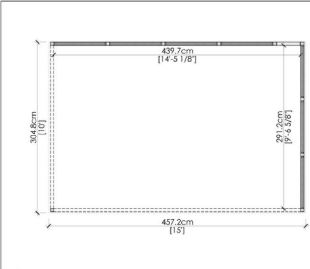
1 TOP VIEW
