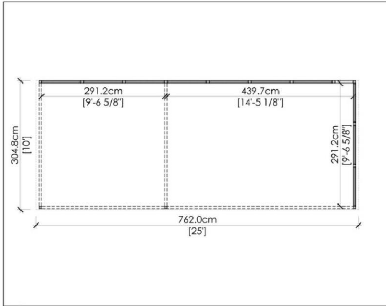
1 TOP VIEW
