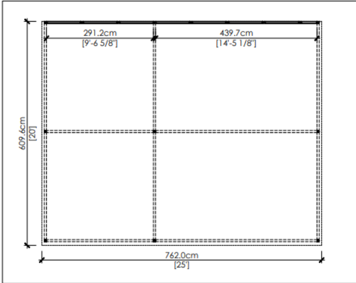
1 TOP VIEW
