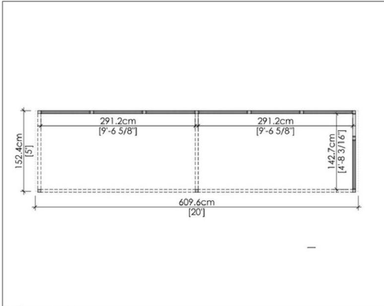
1 TOP VIEW
