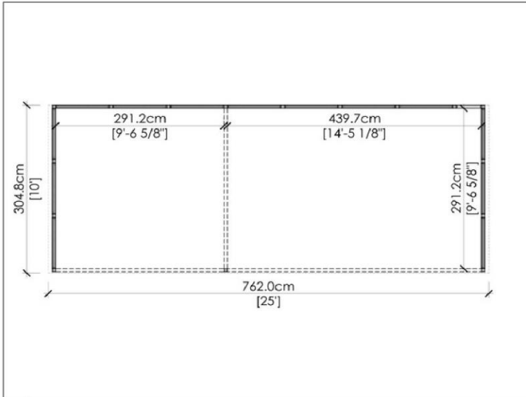
1 TOP VIEW
