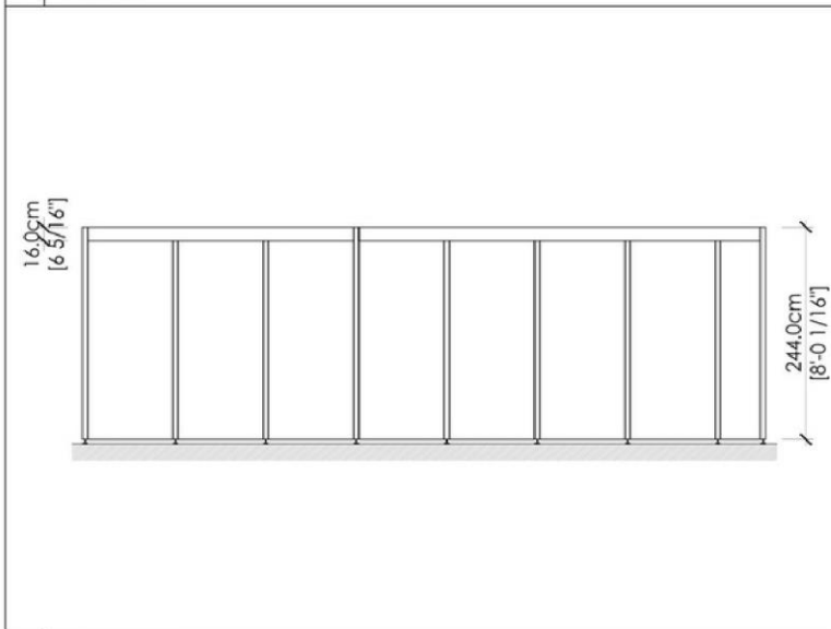
2 FRONT VIEW
