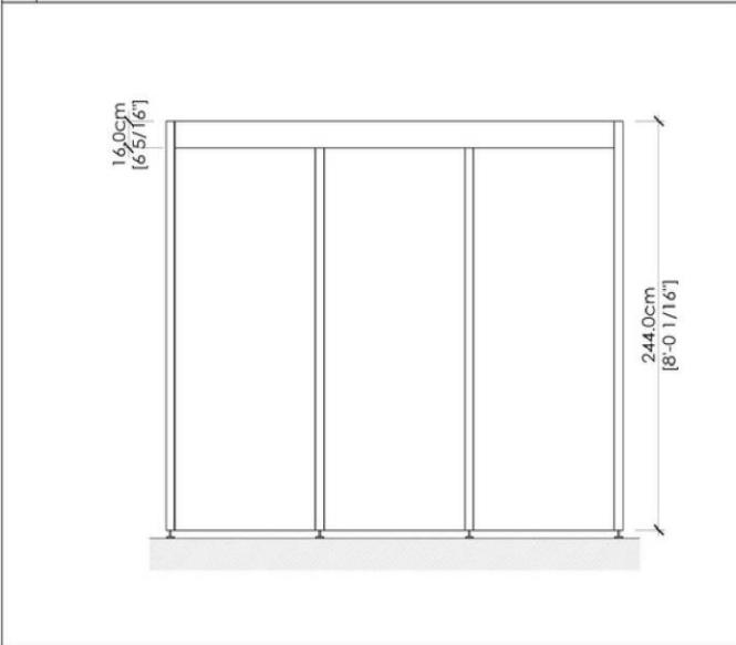
2 FRONT VIEW
