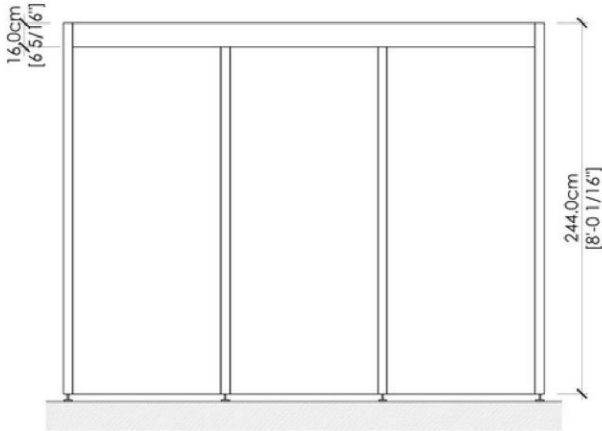
2 FRONT VIEW
