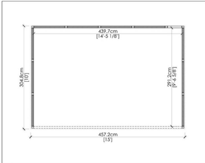
1 TOP VIEW
