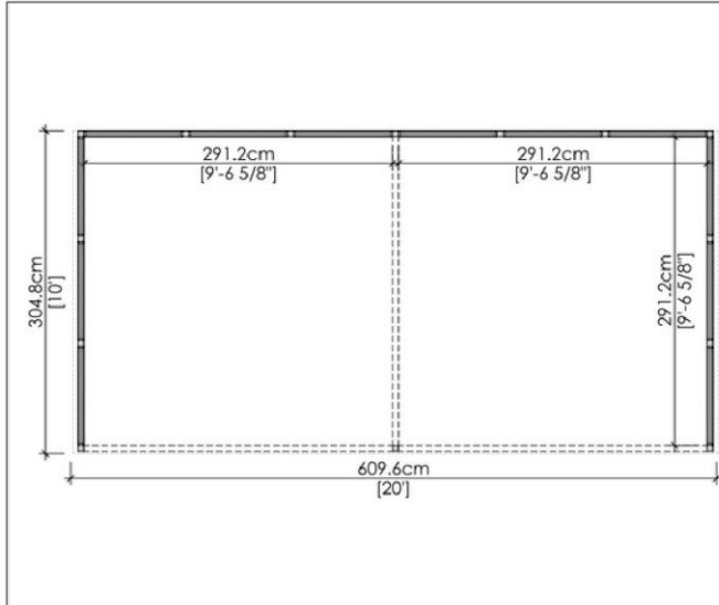
1 TOP VIEW
