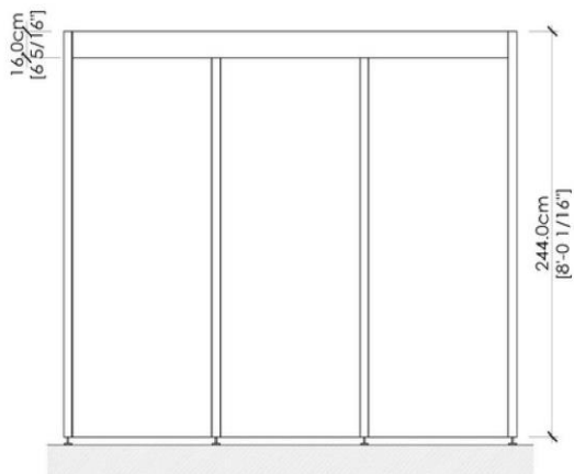
2 FRONT VIEW
