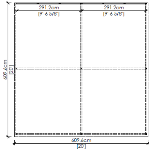
1 TOP VIEW
