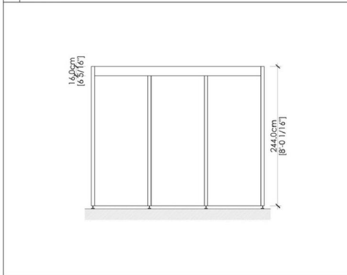
2 FRONT VIEW
