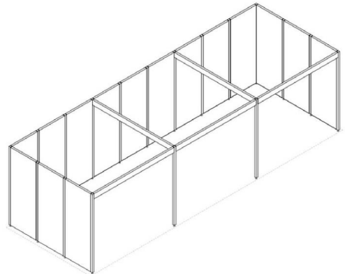
4 3D VIEW
