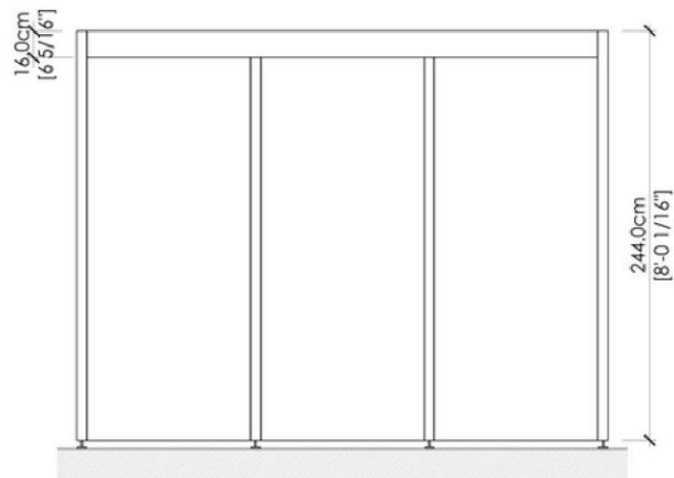
2 FRONT VIEW
