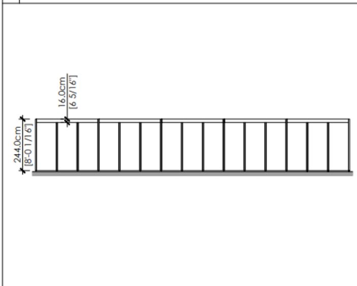
2 FRONT VIEW
